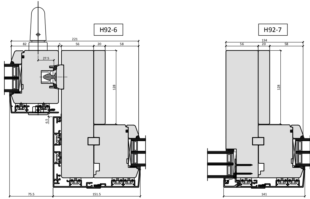
LIFT & SLIDE DOOR COUPLING WITH 92 EUROPA FIXED WINDOW
