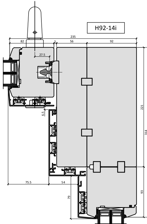
LIFT & SLIDE DOOR COUPLING WITH 92 EUROPA FIXED WINDOW
